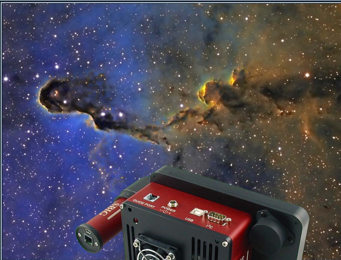
ST-8300 Image of Vdb142 by Peter Clausen
